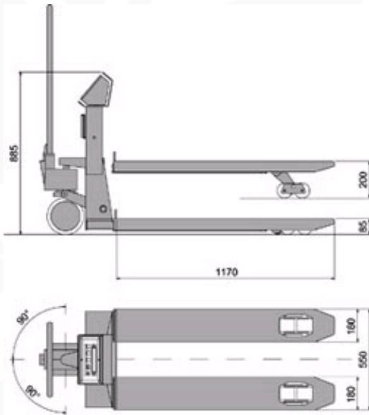
TPWX: Dimensions in mm.
